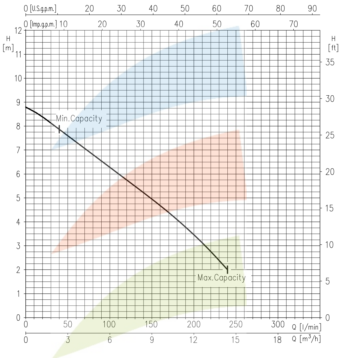
RIGHT 75 (0.55 kW)
