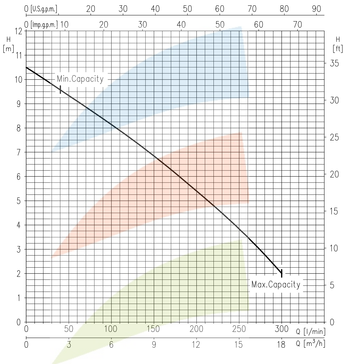
RIGHT 100 (0.75 kW)
